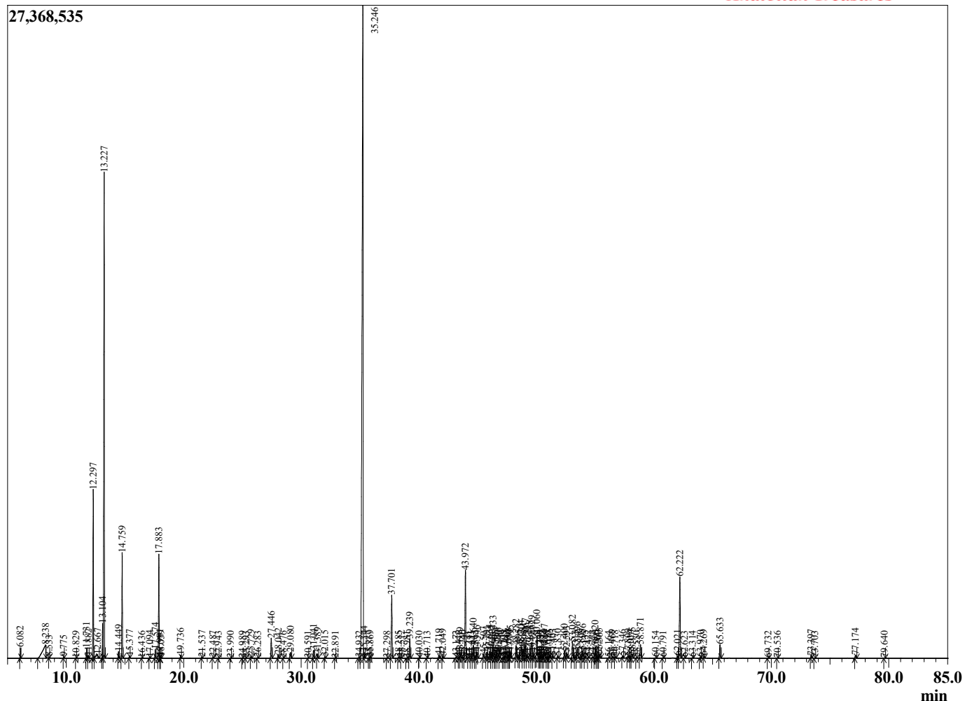
Chromatogram Valeriana officinalis
